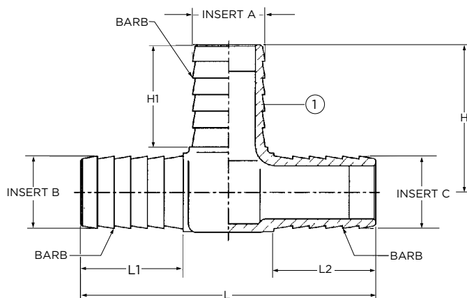
BRONZE INSERT TEE DIMENSIONS (In.)
