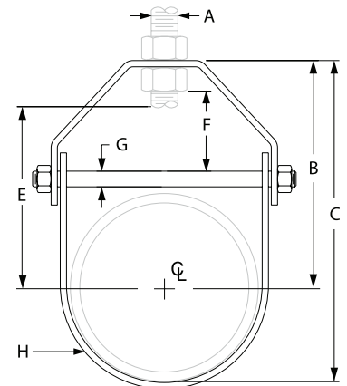
Pipe Sizes 1" and Larger
