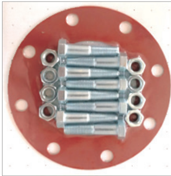
Both ring and full face gaskets are available for ASTM CL 150 and 300 Flanges
