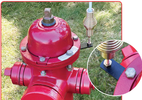
TOP MOUNT MARKERS ATTACH TO THE HYDRANT VIA THE HYDRANT CAP BOLTS.
