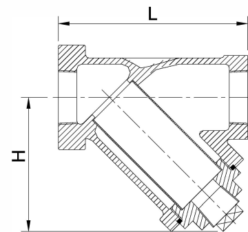
Size DN15-DN50
