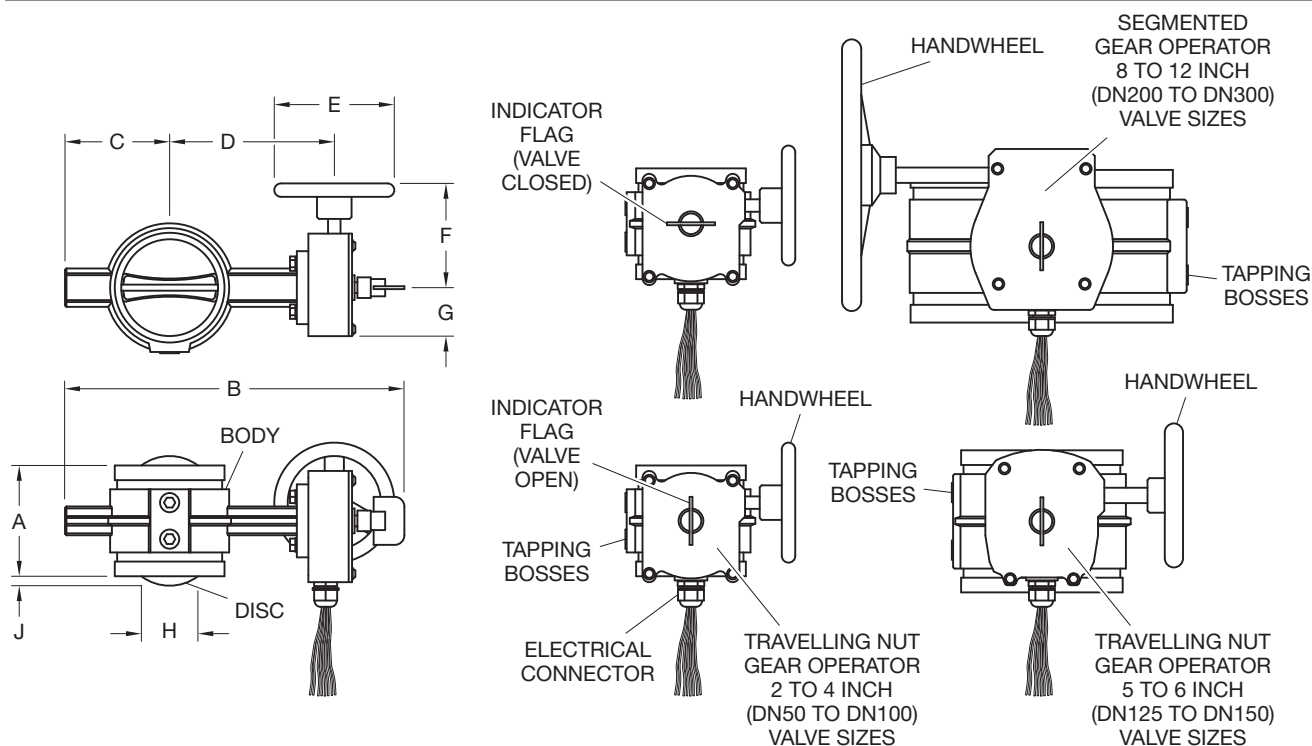
GROOVED END BUTTERFLY VALVE NOMINAL DIMENSIONS
