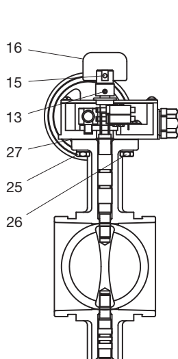
Normally Open Valve Supervisory Switch Arrangement
