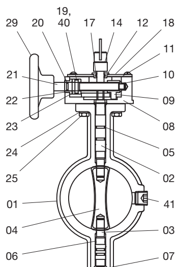
Normally Open Valve Supervisory Switch Arrangement
